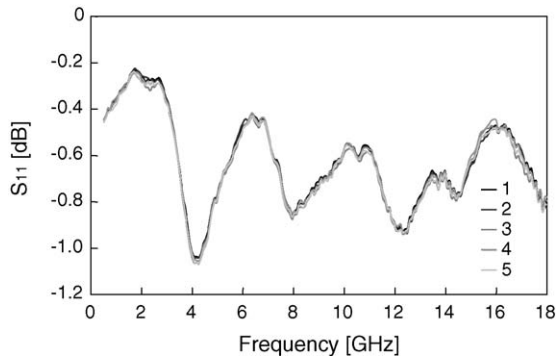
Fig. 9. Measurement reproducibility for the frequency dependence of S_{11} .
