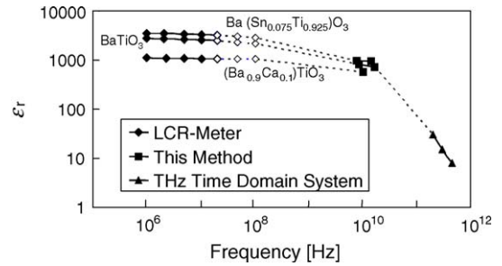
Fig. 8. Dielectric dispersion measured by three different methods.
