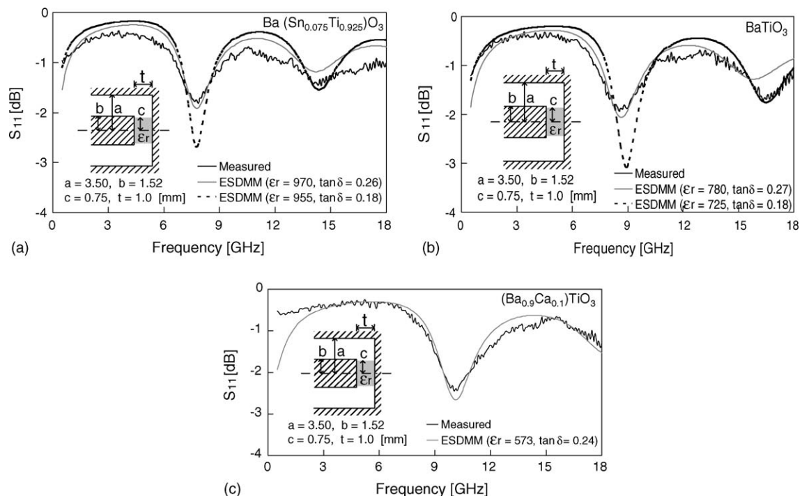
Fig. 7. (a–c) Measured S_{11} and inverse fitting curves of S_{11} with most probable sets of dielectric parameters vs. frequency.
