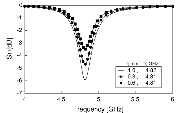
Fig. 5. Dependence of the resonance frequency on the sample height.
